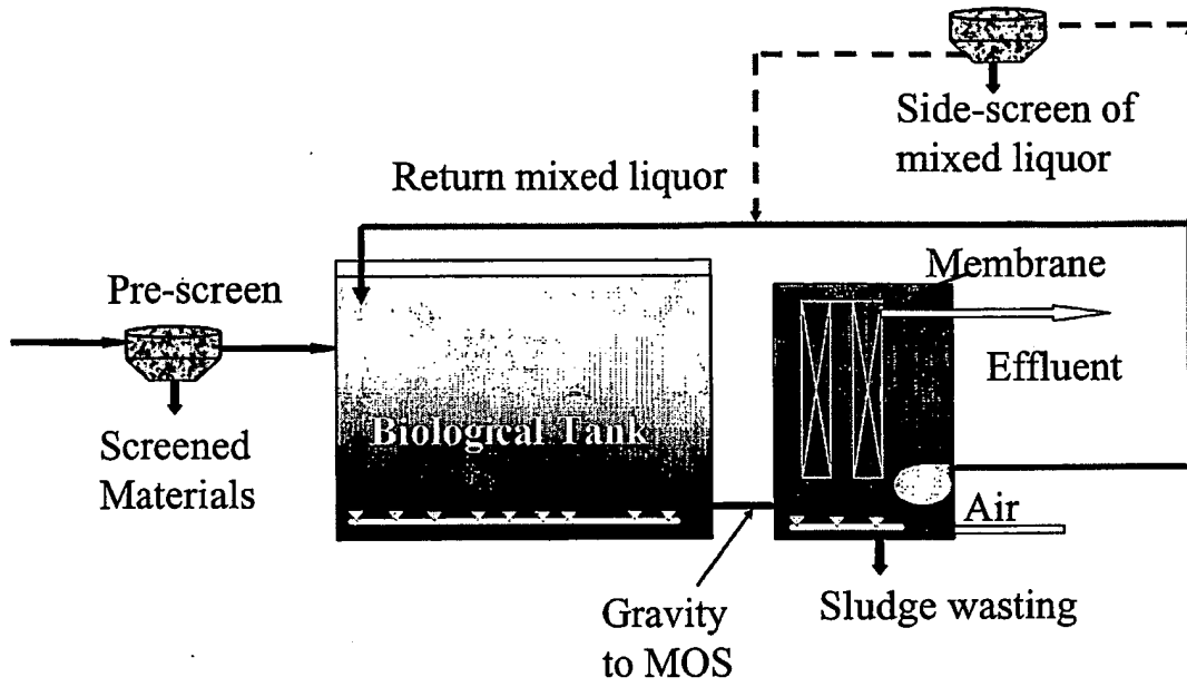
Figure 23 - MBR Configuration with Side Screen in US '868.
